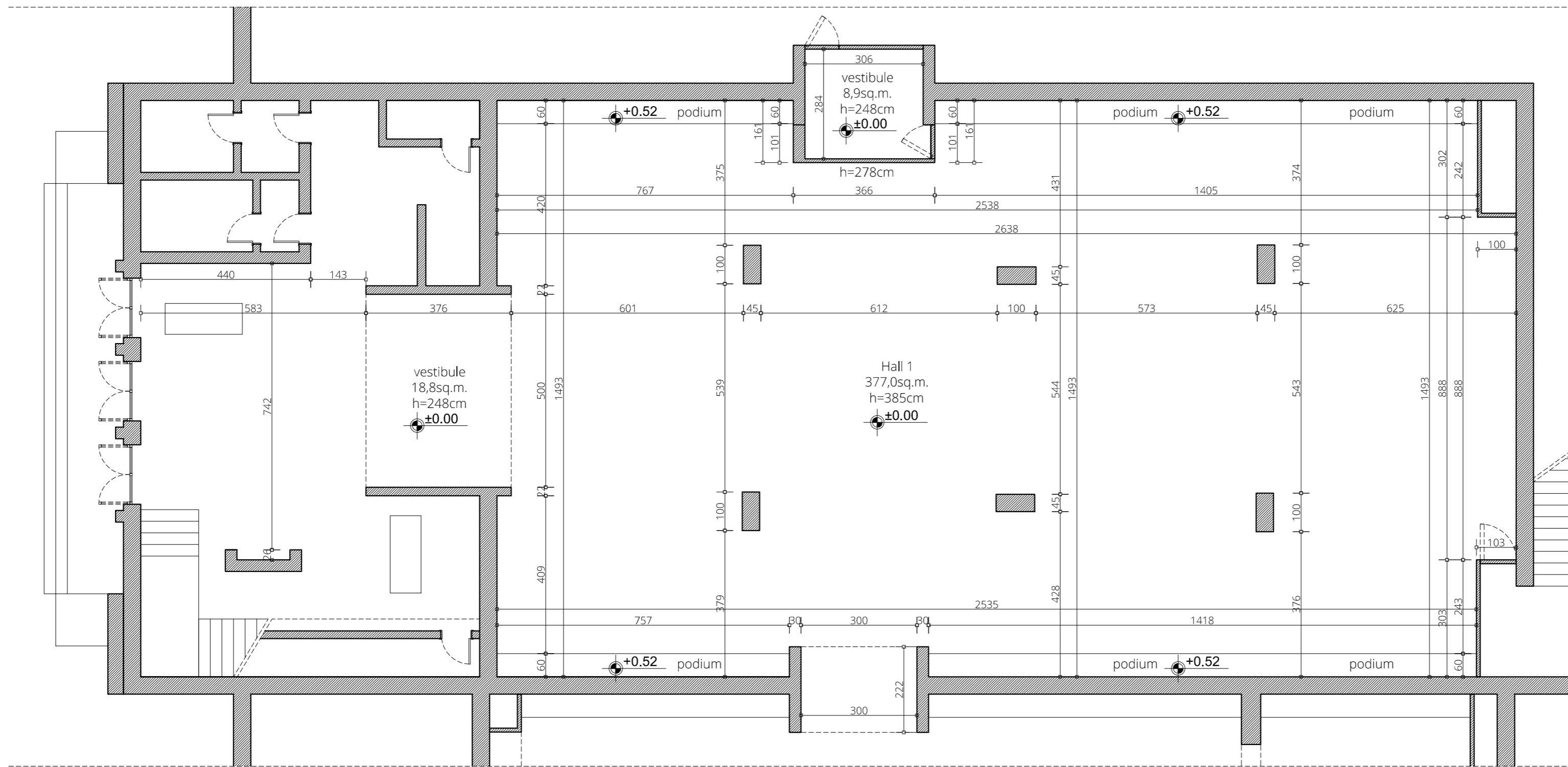
Ground Floor Hall 1 Sc 1:100
