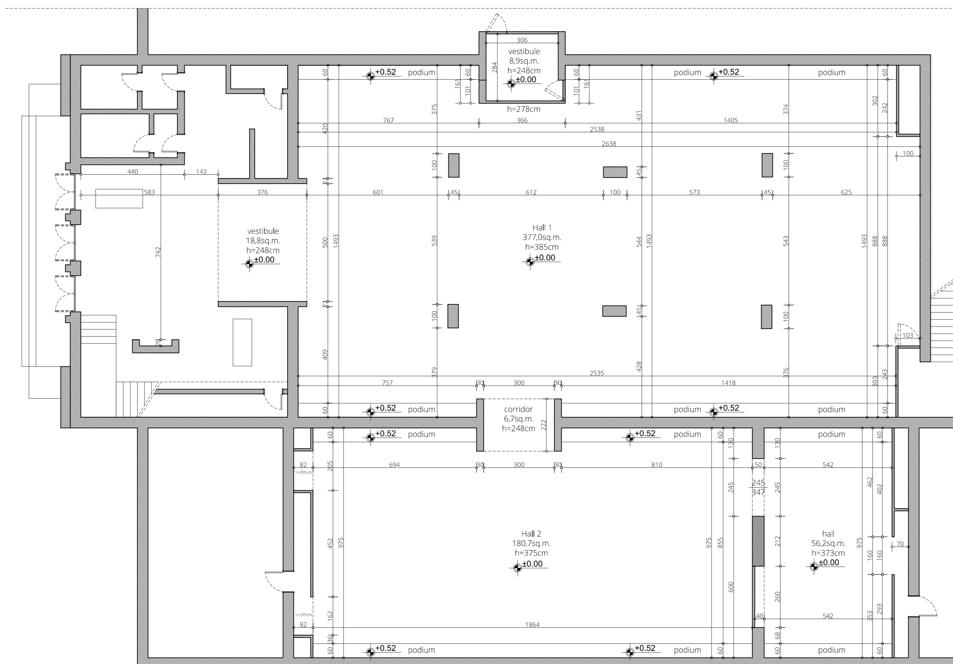
Ground Floor Halls 1 and 2 Sc 1:100
