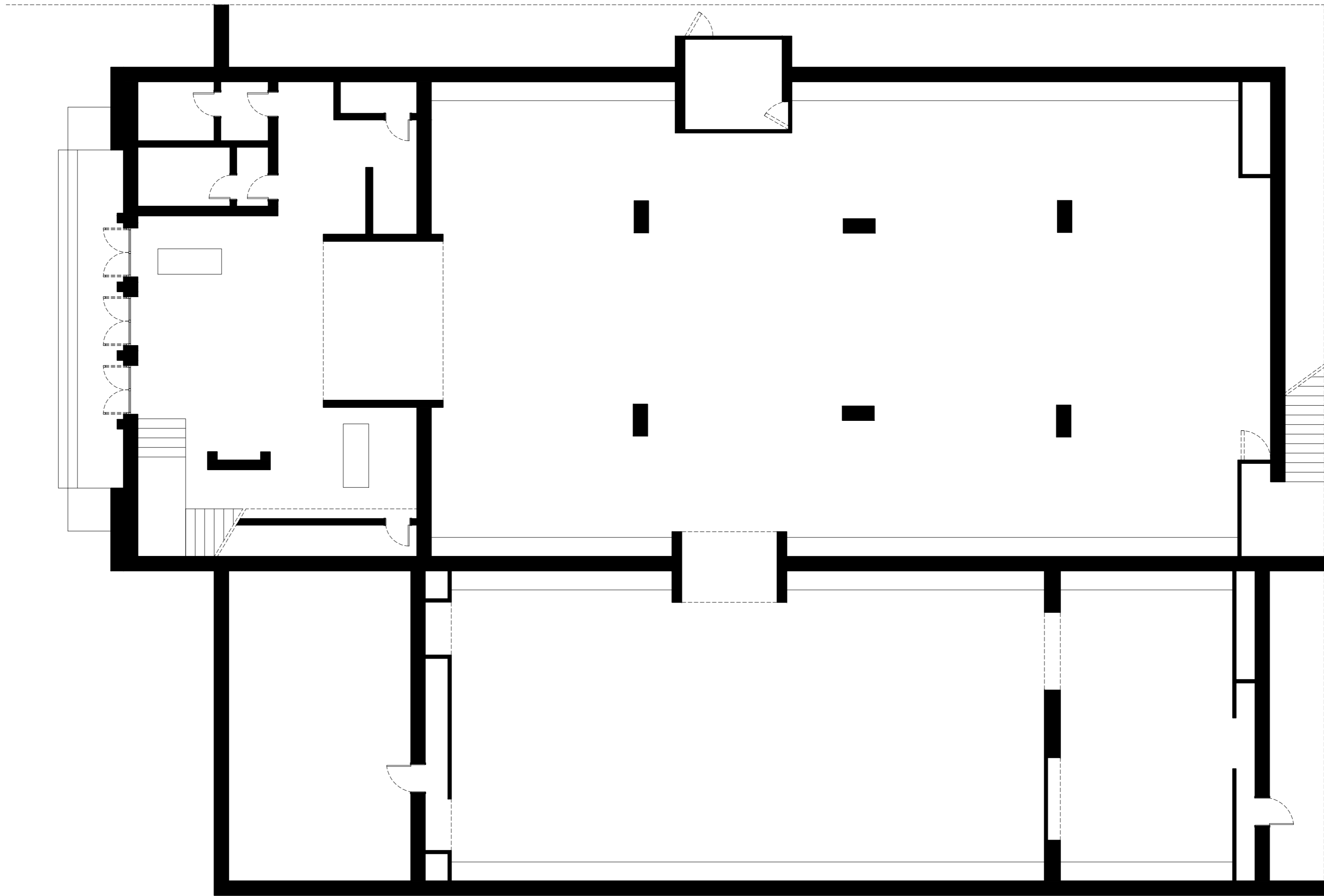
Ground Floor Halls 1 and 2 Sc 1:100
