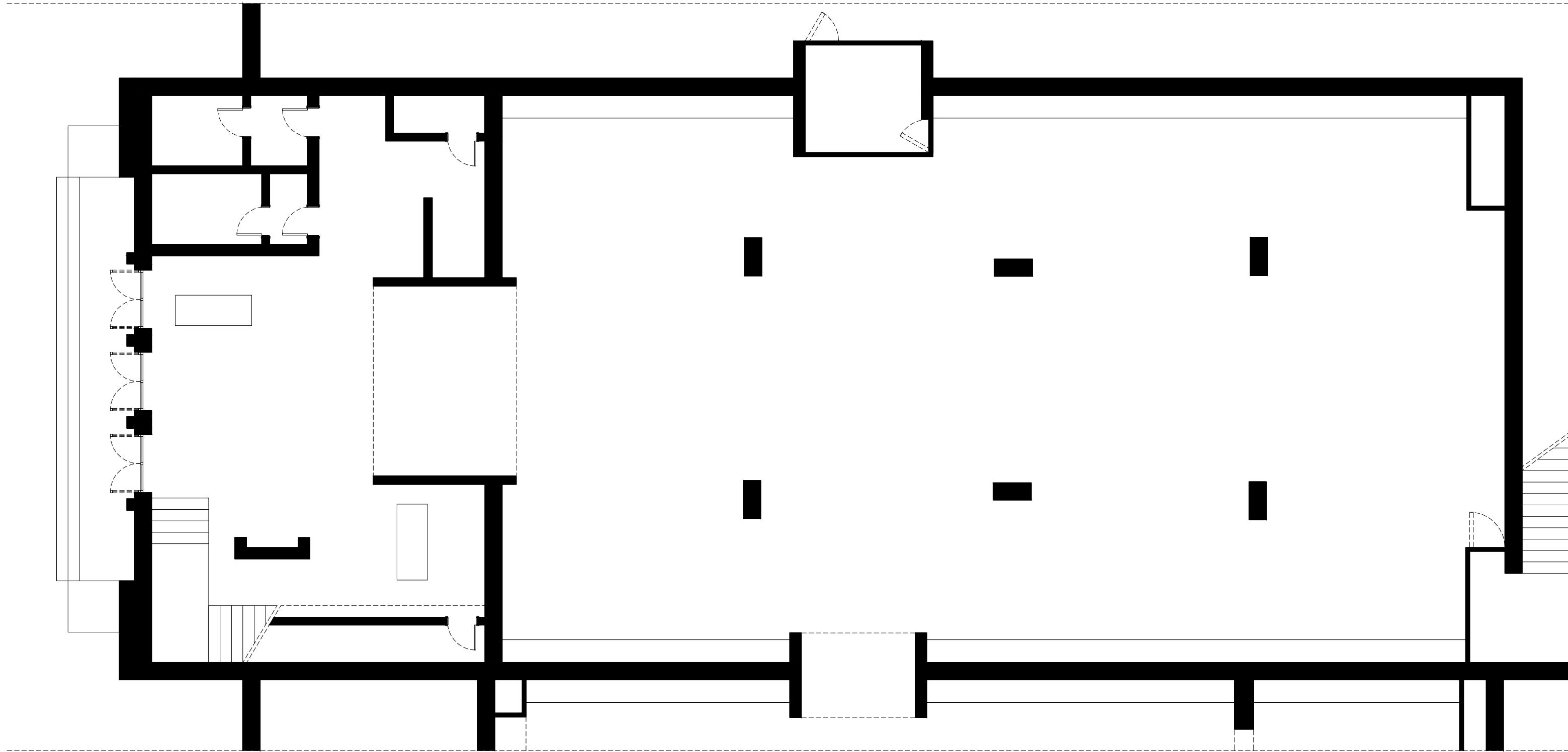
Ground Floor Hall 1 Sc 1:100
