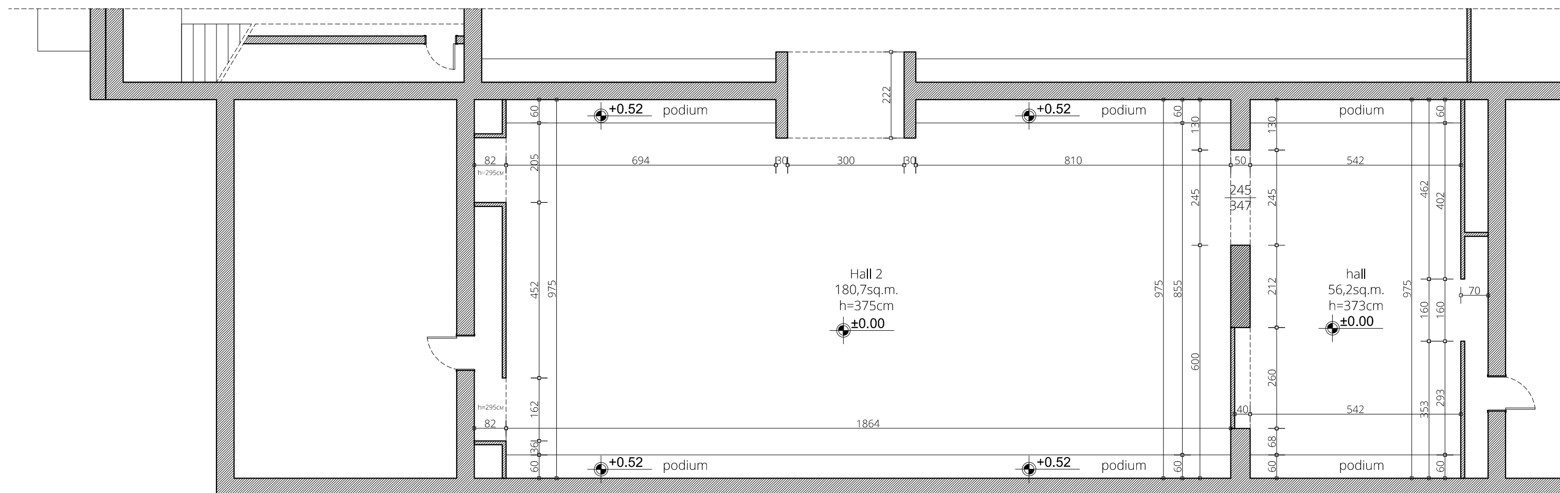
Ground Floor Hall 2 Sc 1:100
