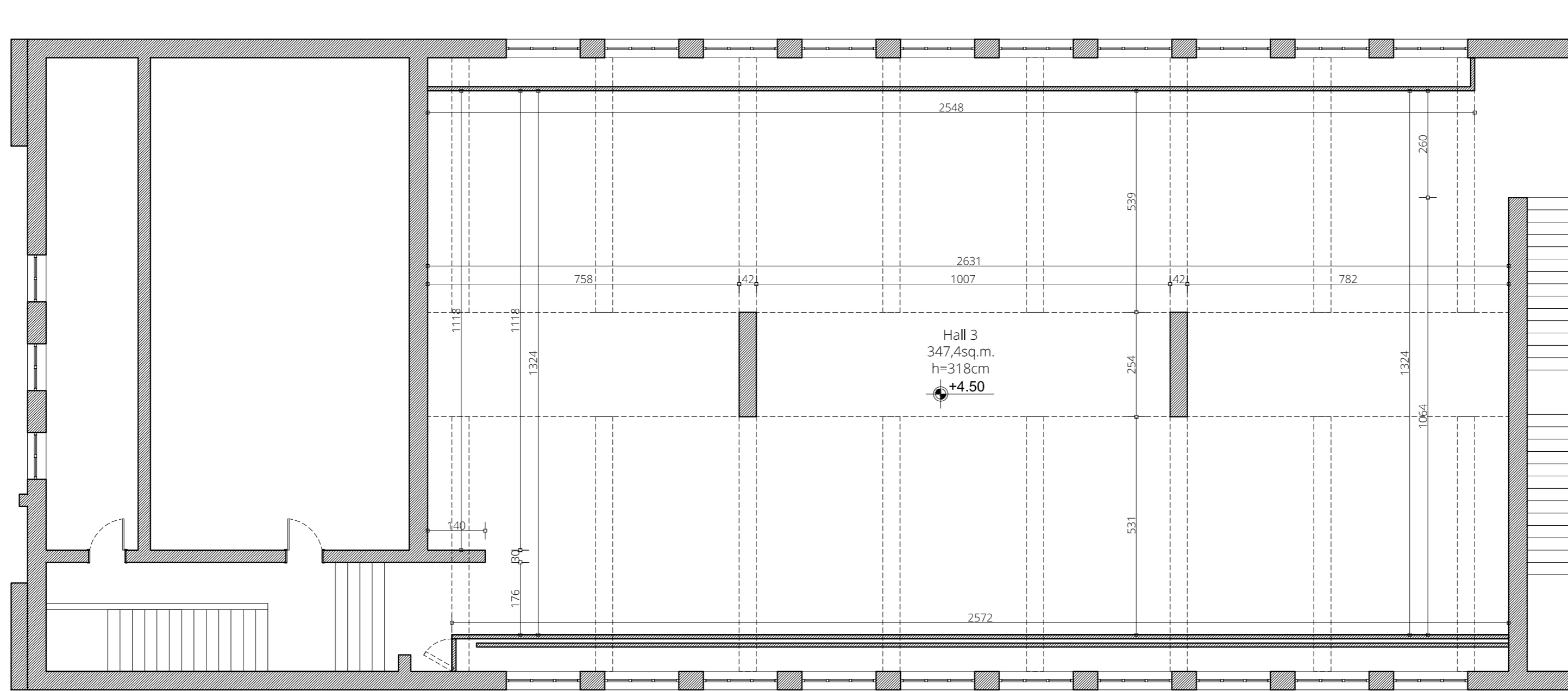
Ground Floor Hall 3 Sc 1:100
